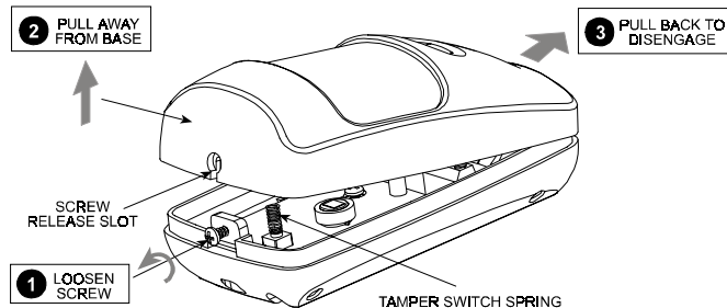
Figure 3. Cover Removal
